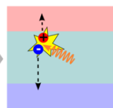
reabsorption
