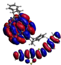
internal emission
