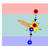
internal emission
