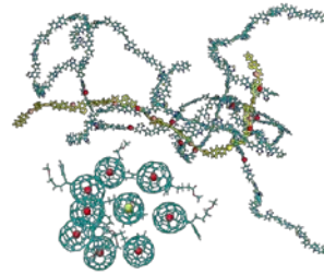
reabsorption
